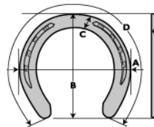
Euro Side Clipped - Lite Hind
