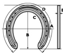
American Aluminum Racing Plates Hind
